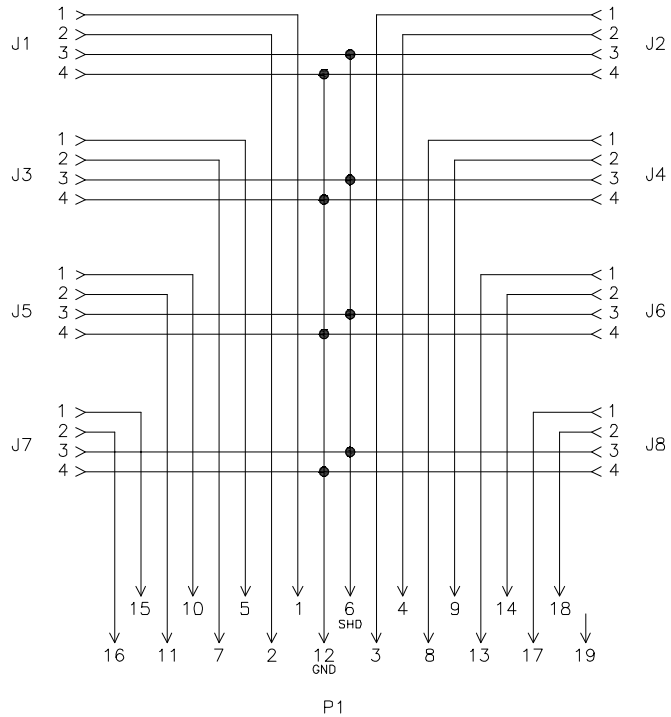
WIRING DIAGRAM SOURCE DRAWING - FOR REFERENCE ONLY
